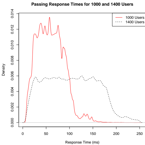
Fig. 2. Density functions of passing response times in milliseconds for 1000 and 1400 users on a cluster of 40 nodes (ms)
