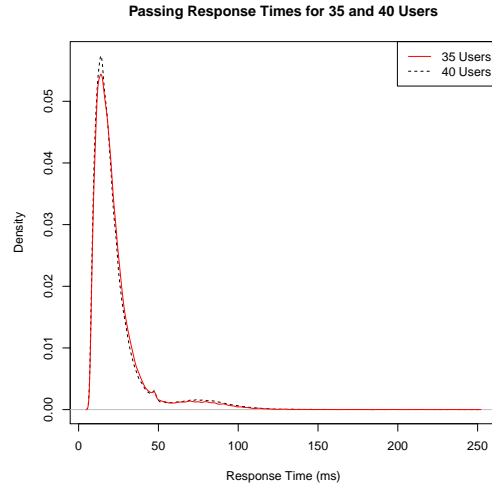
Fig. 1. Density functions of passing response times in milliseconds for 35 and 40 users on a single node (ms)
